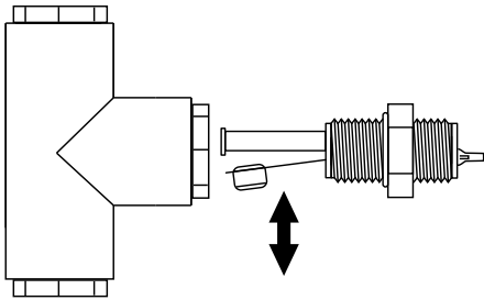
FS-PT-P Paddle style flow switch assembly. Comes with 1" PVC tee; 150 psi @ 75°F.
