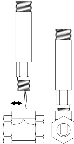
FS-HP1 Paddle style flow switch. High pressure, 1" brass, 250 psi
