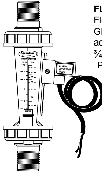
FS-OC Cap & float style flow switch comes with 3/4" PVC tee; 140 psi @ 75°F
