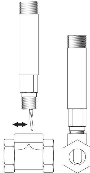
FS-HP-075 Paddle style flow switch with 3/4" brass tee, 250 psi @ 220°F.
